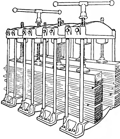
FIG. 412. VENEER PRESS.
